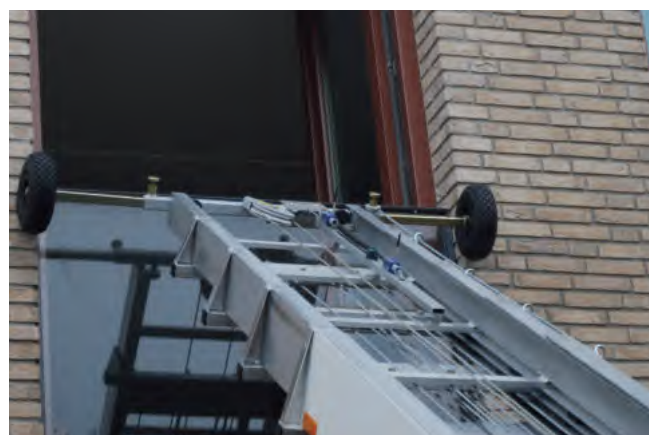
Wheels at head section adjustable
